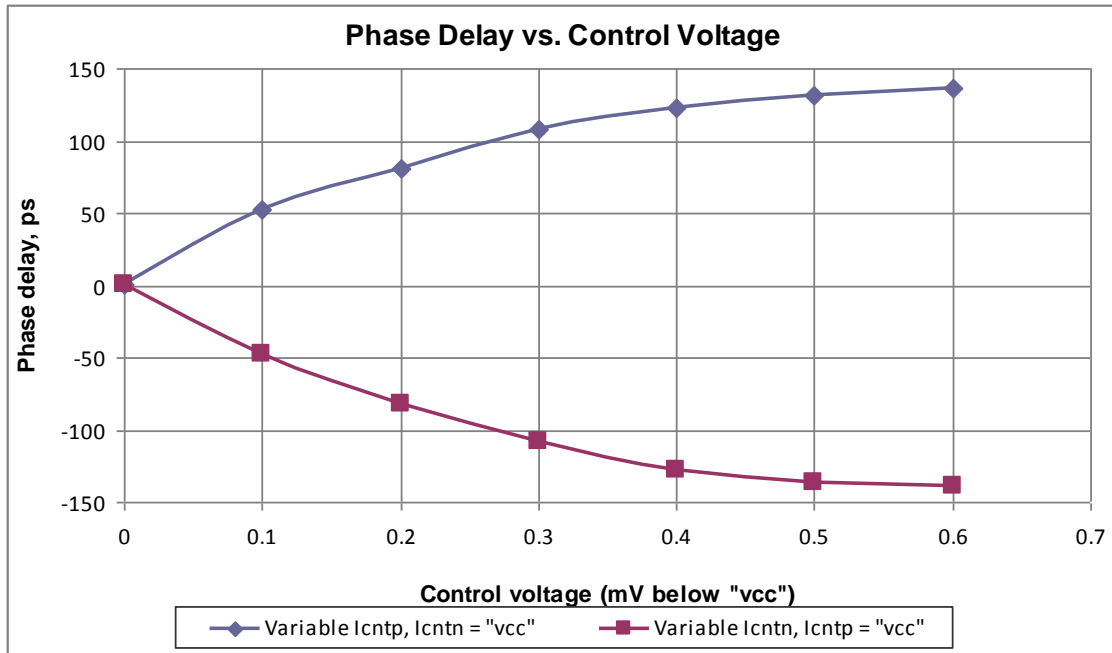
Fig. 2. Delay Control Diagram
