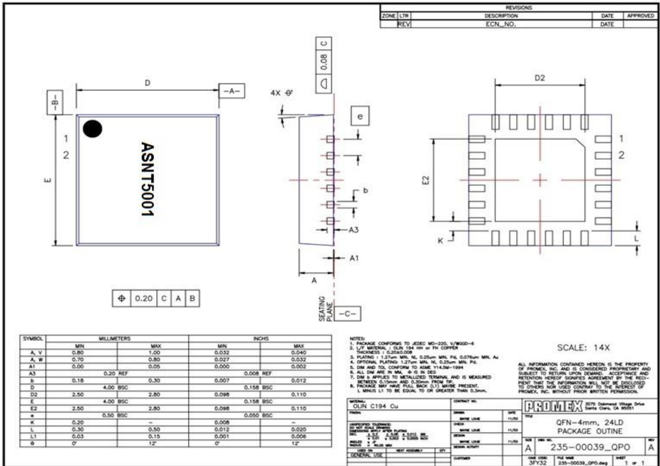
Fig. 3. QFN 24-Pin Package Drawing (All Dimensions in mm)
